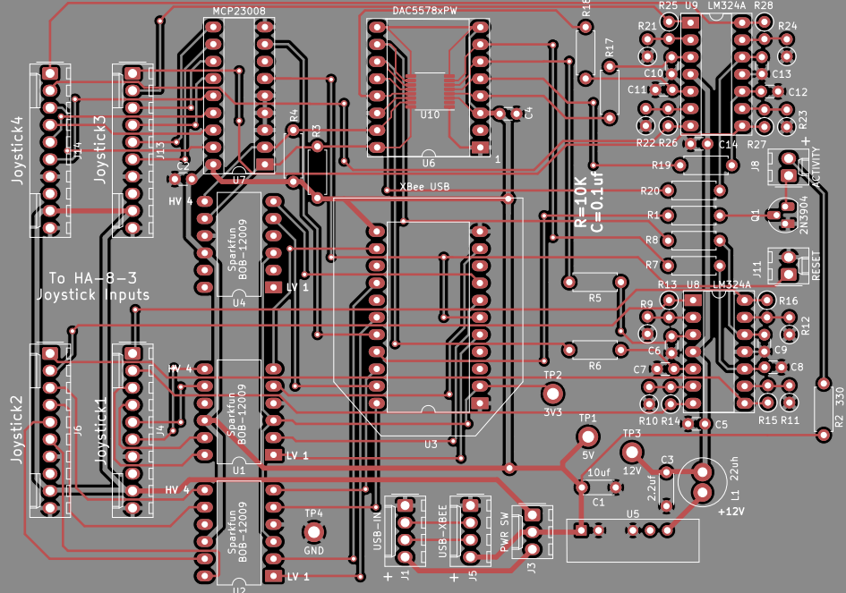
4-CHANNEL RF JOYSTICK RECEIVER FOR HA-8-3 COLOR GRAPHICS CARD
